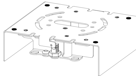
directly to the ceiling *use appropriate anchors
