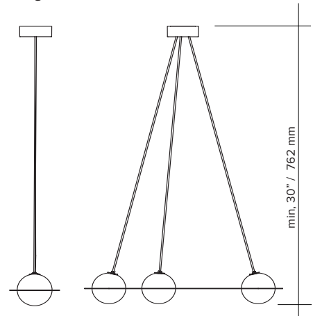
angled wires
