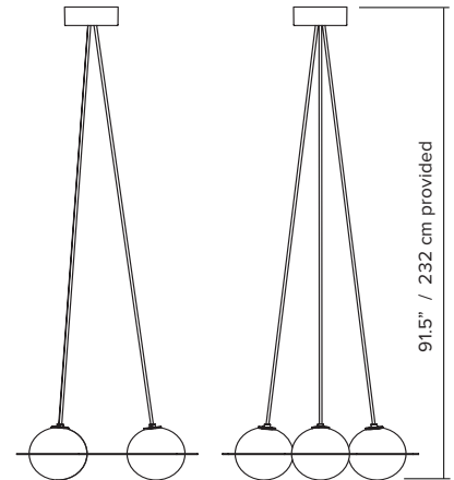
angled wires
