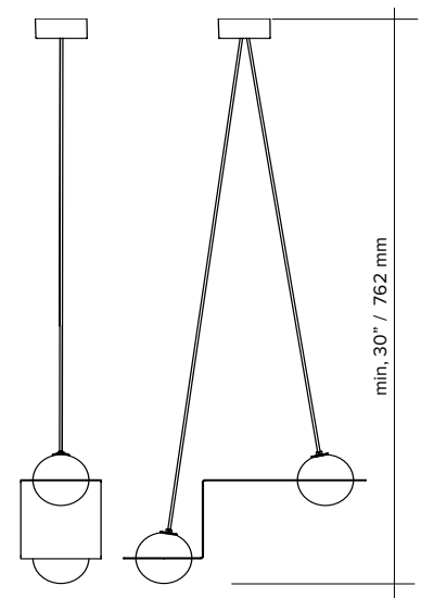
angled wires
