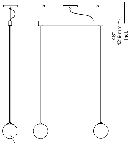
parallel wires with offset connection
